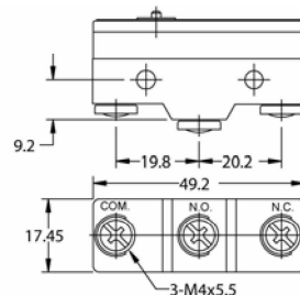
Screw Terminal
